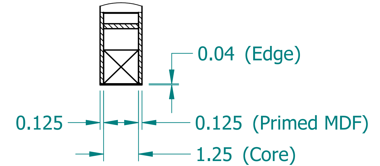
DETAIL B
